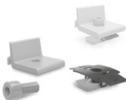
K2 Climber 36/50 Set
